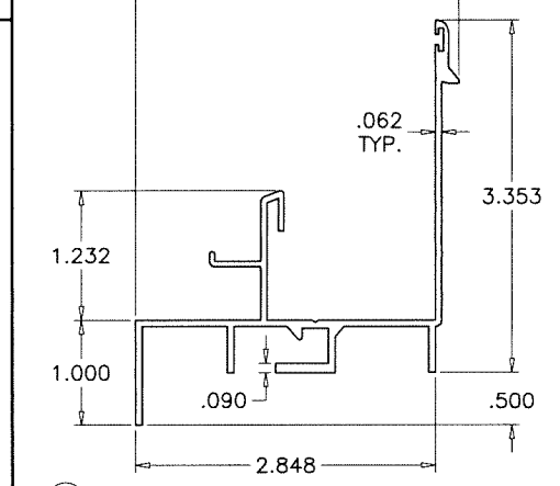
② FRAME SILL
