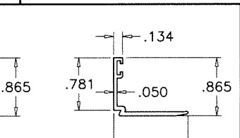
⑧A GLAZING BEADS
