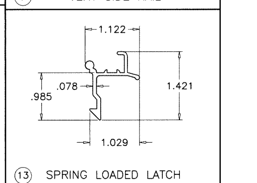
⑬ SPRING LOADED LATCH
