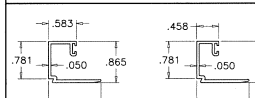
⑧ GLAZING BEADS
